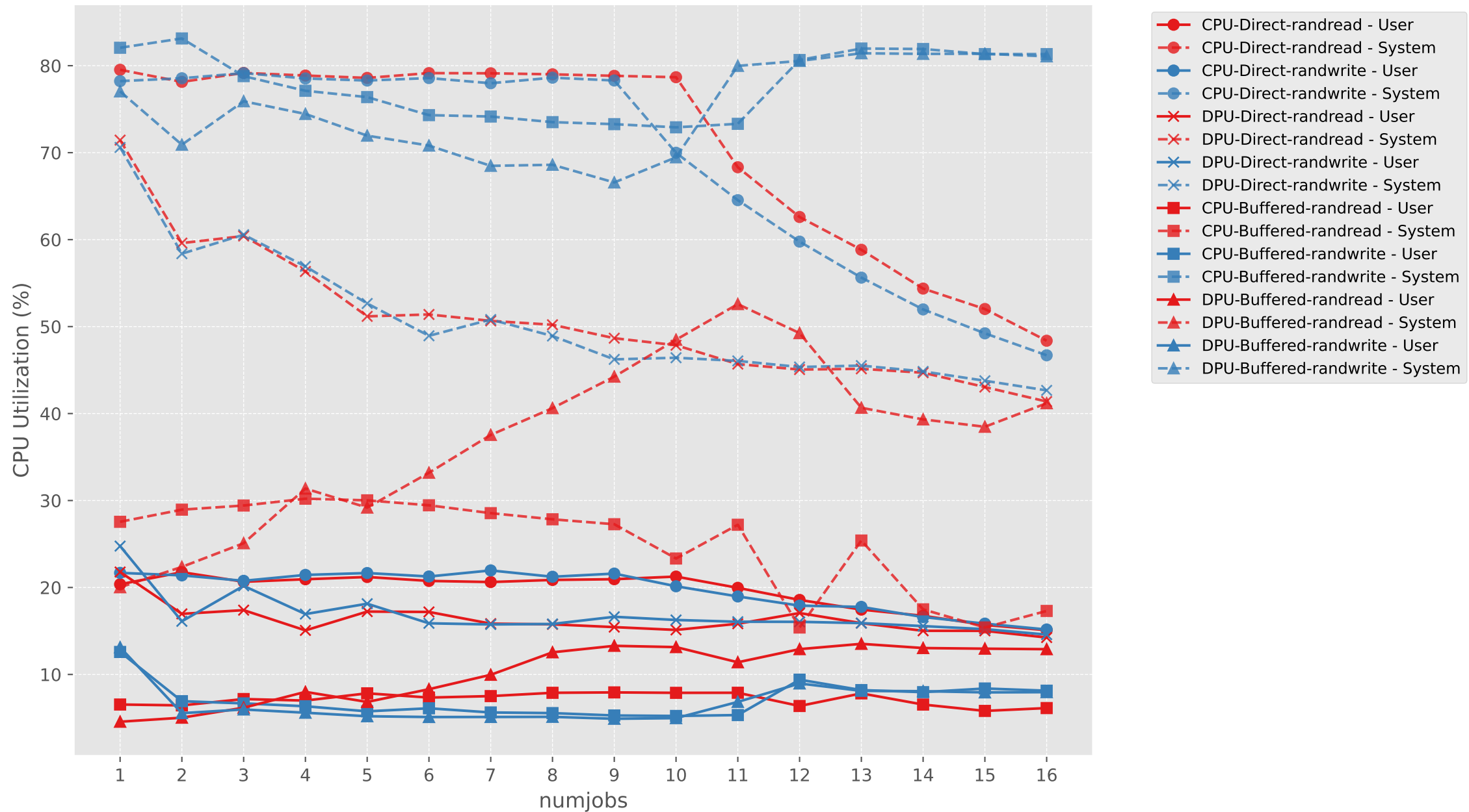
CPU Utilization vs numjobs (CPU vs DPU, Direct vs Buffered)
